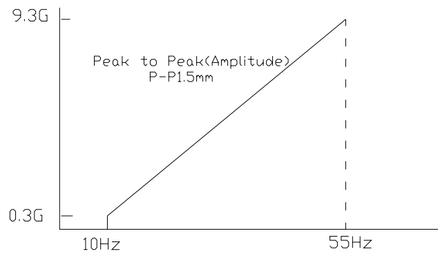
FIG3 VIBRATION TEST
