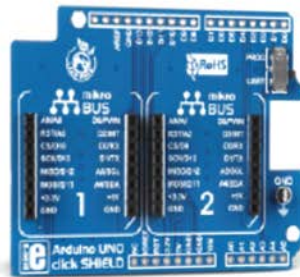
click shields (12)
